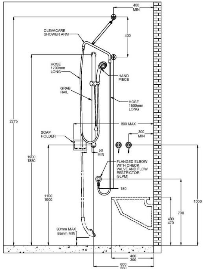
Clevakit typical installation Conforming to AS1428.1-2009
